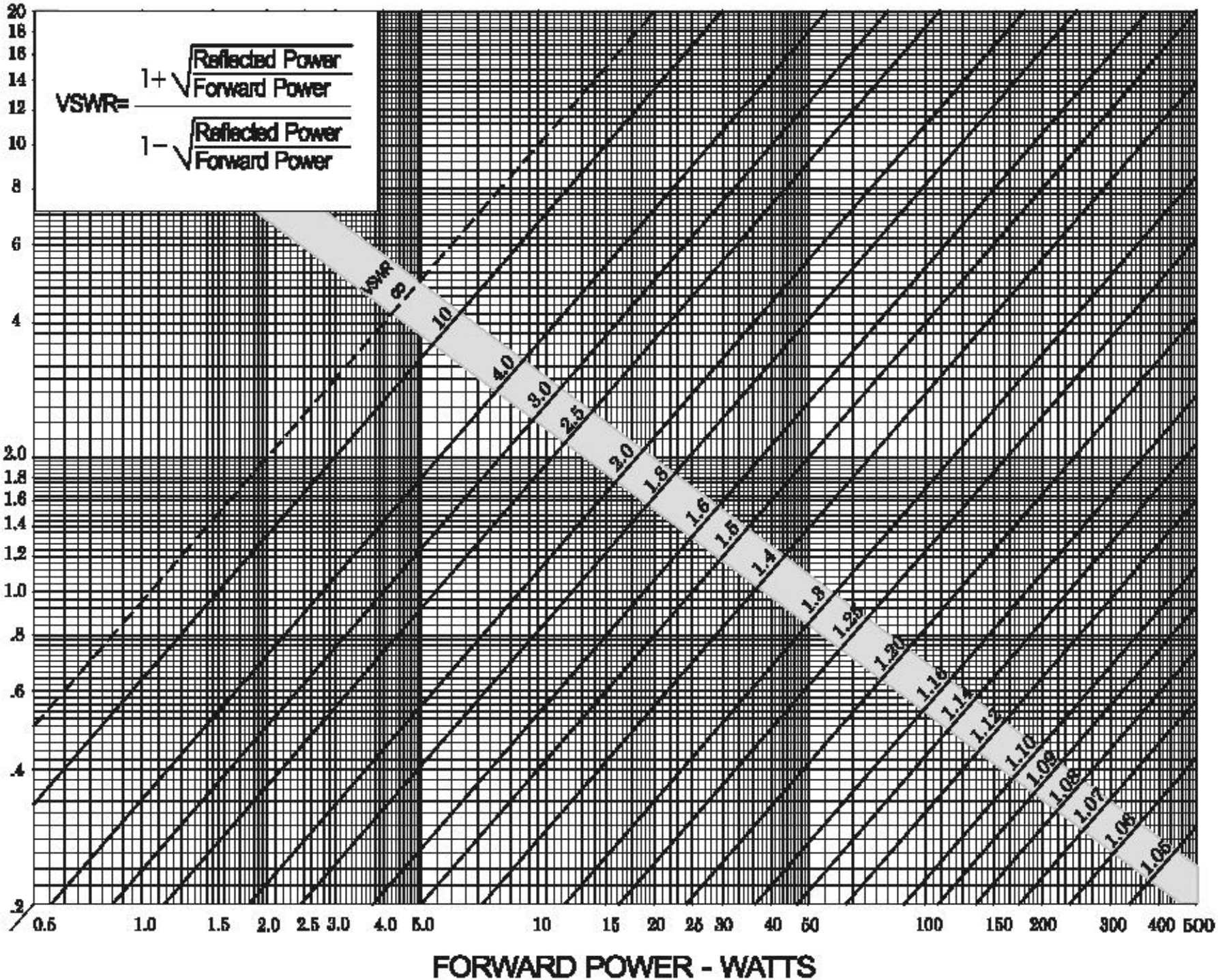
VSWR Conversion Graph (Reflected Power 0.2 – 20.0)
