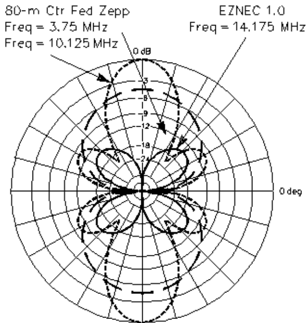
Azimuth Plot Elevation Angle = 30.0 deg
