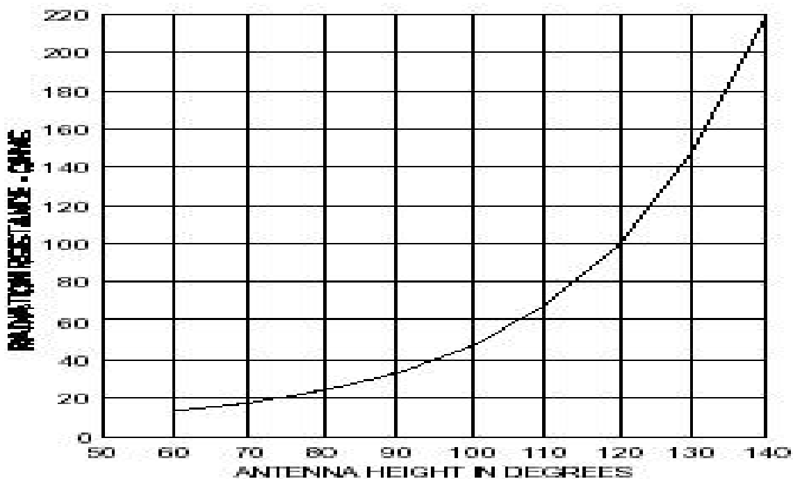
Fig. 49 — Radiation resistance versus free space antenna height in electrical degrees for a vertical antenna over perfectly conducting ground, or over a highly conducting ground plane. This curve also may be used for center-fed antennas (in free space) by multiplying the radiation resistance by two; the height in this case is half the actual antenna length.
