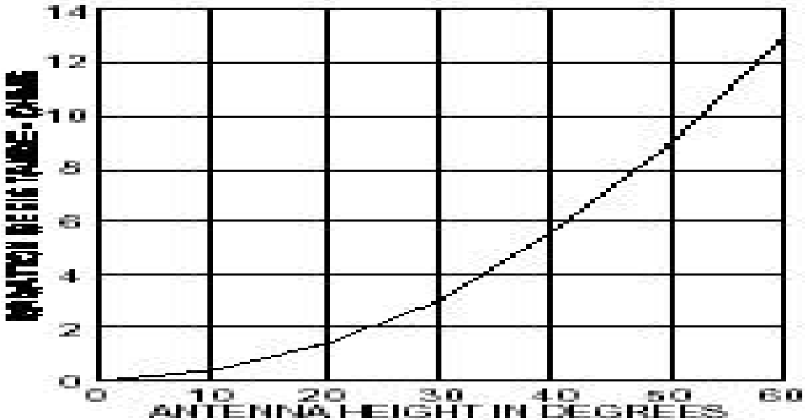
Fig. 50 — Same as Fig. 49, for heights below 60 degrees.
