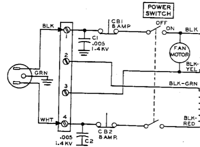
SCHEMATIC OF THE HEATHKIT® LINEAR AMPLIFIER MODEL SB-200
