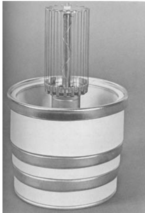
Figure 19: Typical bar tungsten filament
